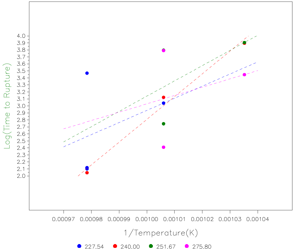
For Set1 LOG(TIME) vs 1/Temp(K)
