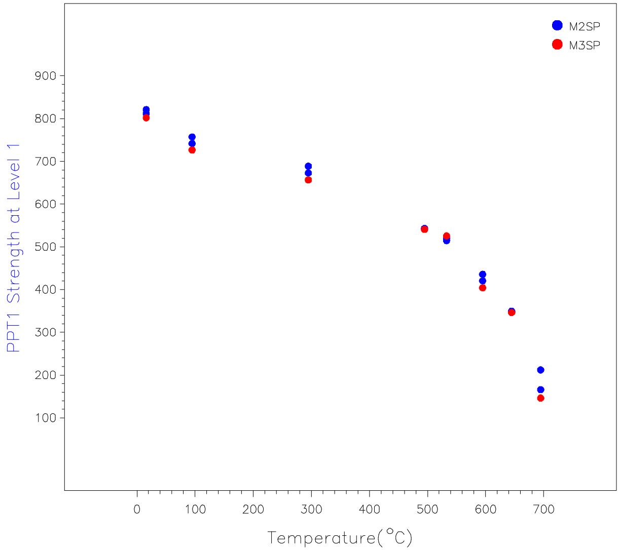
PPT1L1 Strength vs Temperature (for SP Method)
